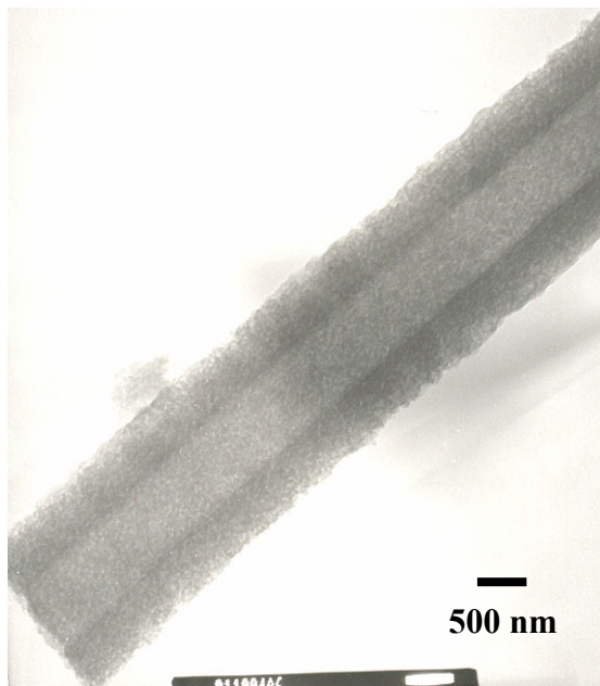
Fig. S1 TEM image of carbon tube showing disordered mesoporous walls.
